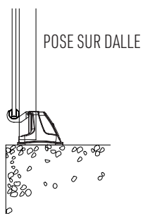
Sabot standard
