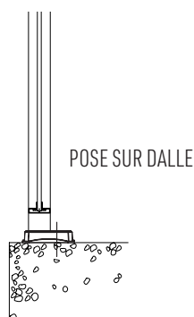
Sabot standard
